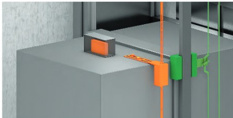
Shaft copying system with stainless steel coded band. Control boxes with certified evaluation unit (PSU).
